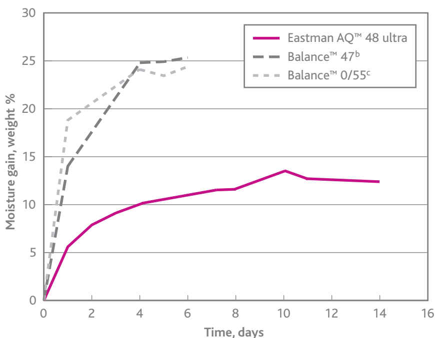
Figure 2 Moisture regain of Eastman AQ™ 48 ultra and acrylic polymers a
