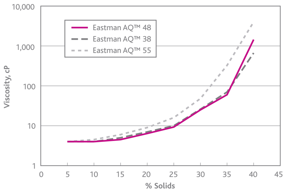
Figure 4 Viscosity of Eastman AQ™ aqueous dispersions
