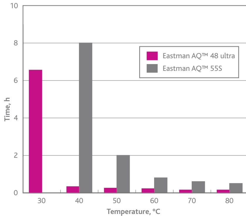
Figure 3 Effect of temperature on dispersion rate of Eastman AQ™ 48 ultra and 55S polymers
