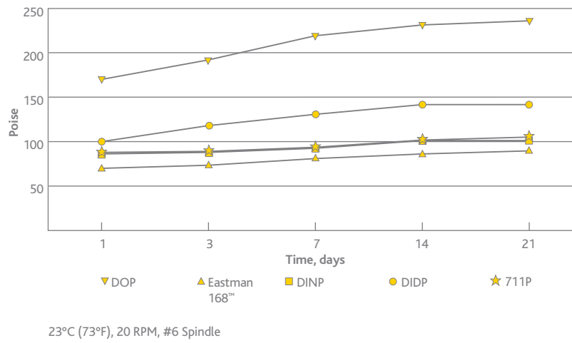
Figure 3 Brookfield viscosity
