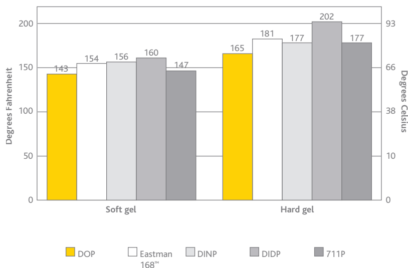
Figure 6 Fusion properties of plastisols
