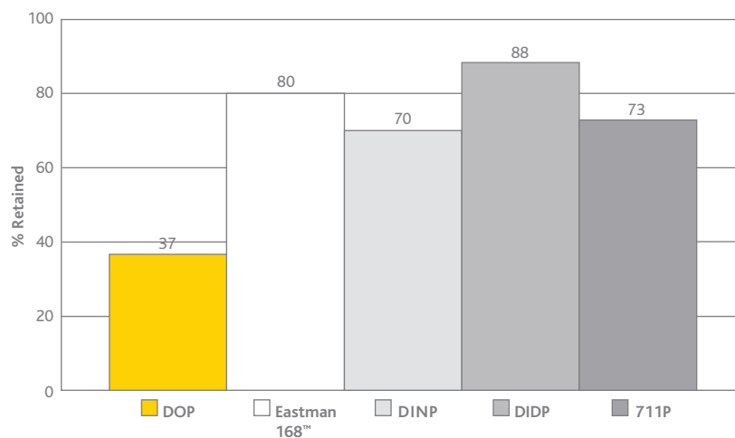
Figure 2 Plasticizer volatility
