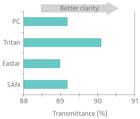
Figure 1 Total light transmittance of clear materials
