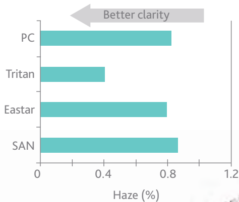
Figure 2 Haze analysis of clear materials
