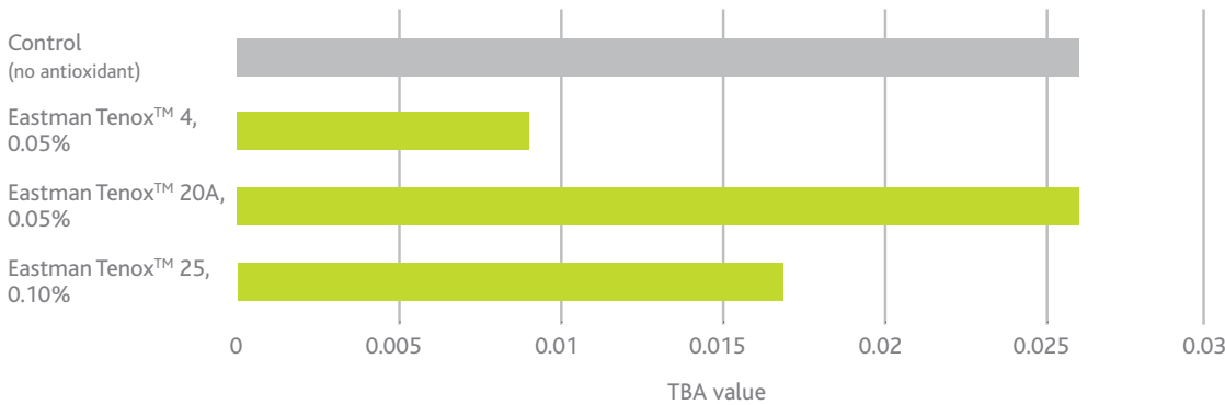
Figure 3 TBA values for sausage a Duncan’s multiple range test
