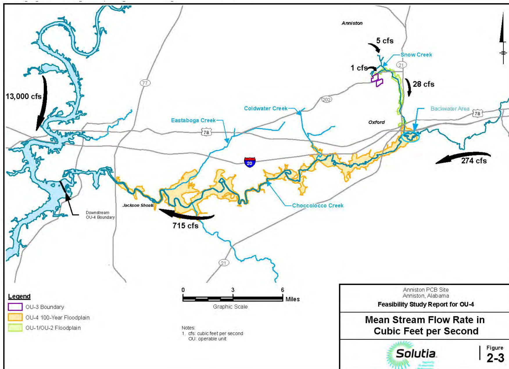
Figure 4. Mean Stream Flow Rate in Cubic Feet per Second
