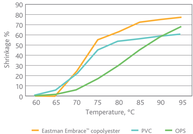
Shrink rate comparison curves (10 sec)
