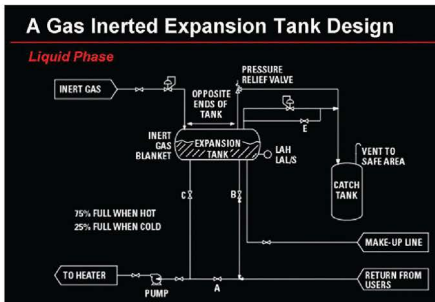
FIGURE 1. Shown here is a basic design for an expansion tank. A preferred design for an expansion tank is one with a double-drop-leg arrangement, where the diameter of the drop-leg piping is as close to the same size as the return header as possible. This design allows for full fluid flow through the expansion tank during startups and during times when moisture or low boilers must be vented from the system.
