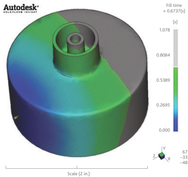
Figure 3 Computer-aided mold filling analysis image
