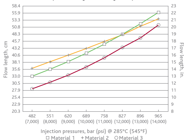
Figure 1 Spiral flow data at midrange temperatures (3.2-mm [0.125-in.] wall)
