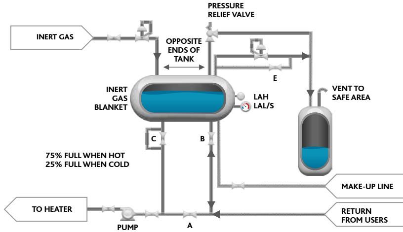
Figure A. Suggested inert gas arrangement for expansion tank
