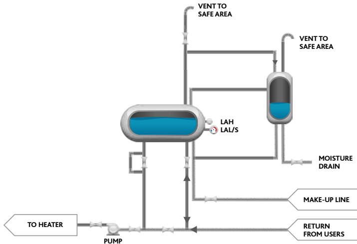
Figure B. Suggested cold seal trap arrangement for expansion tank
