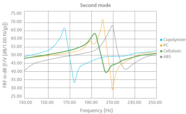
Figure 3b. Modal resonance—detail
