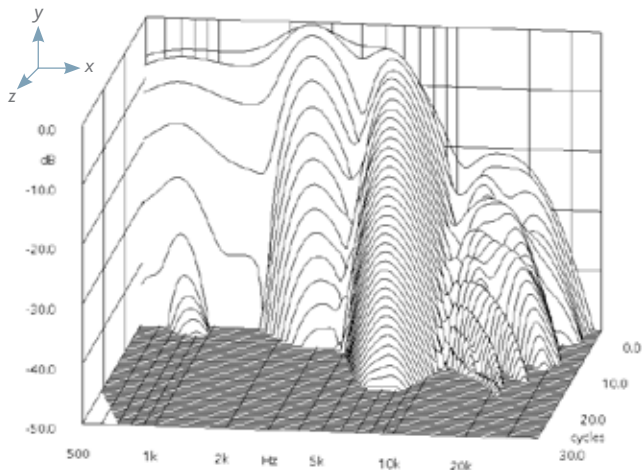
Figure 5b. Copolyester
