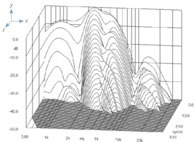
Figure 5c. Cellulosic
