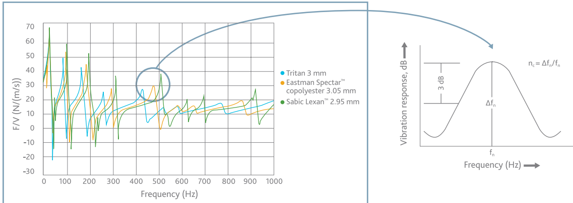
Figure 3b. Modal resonance—detail
