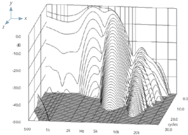
Figure 5a. Polycarbonate
