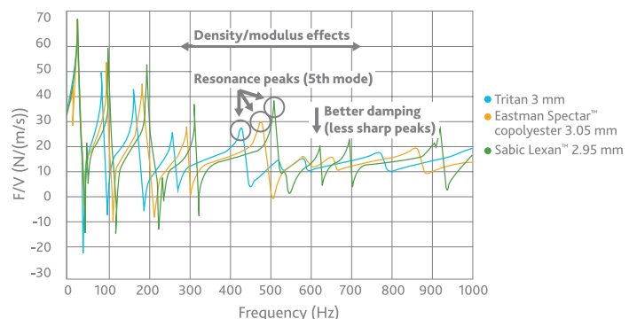
Figure 2. FRF example
