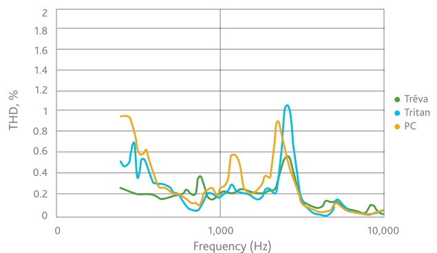
Figure 6. THD @ 100 dB SPL, IEM
