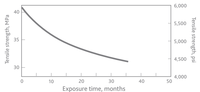
Figure 1. Tensile strength at break of Tenite™ butyrate weathered in Arizona
