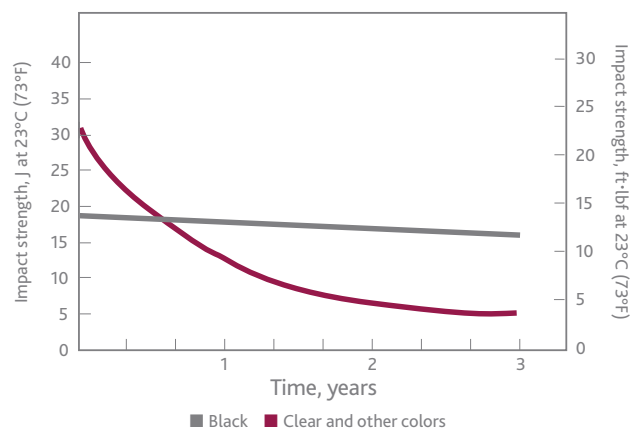
Figure 3. Plaque impact strength (ASTM D3029) of weathered Tenite™ butyrate struck on weathered side
