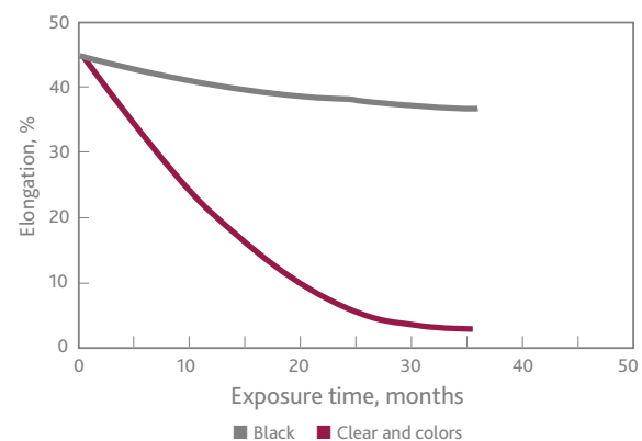
Figure 2. Elongation at break of Tenite™ butyrate weathered in Arizona
