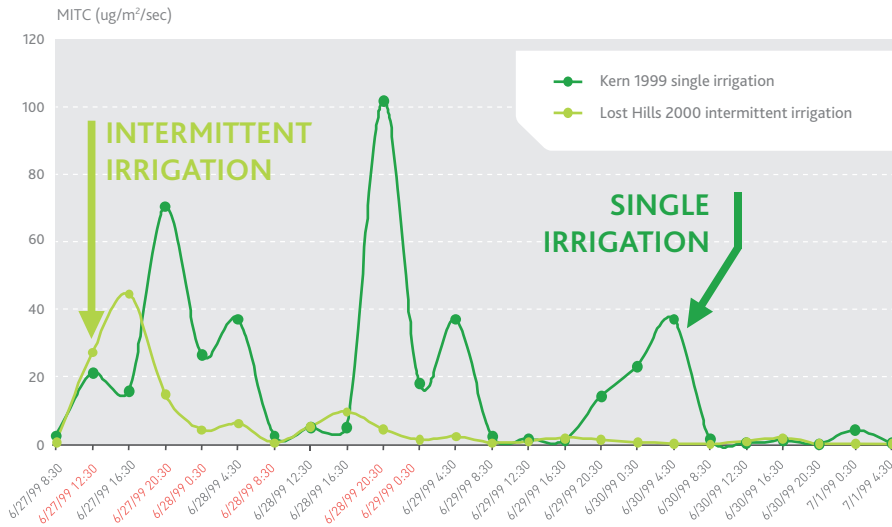
Comparison of MITC flux to the atmosphere during a 96-hour monitoring period with 24 samplings with 4-hour intervals between intermittent irrigated and single irrigated metam-treated fields.
