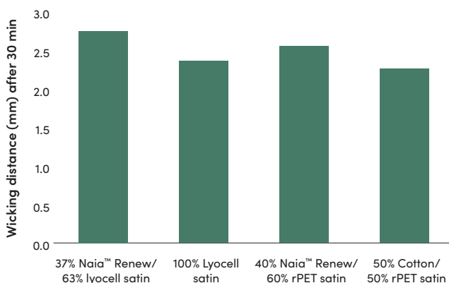
Drying rate AATCC 201-2014
