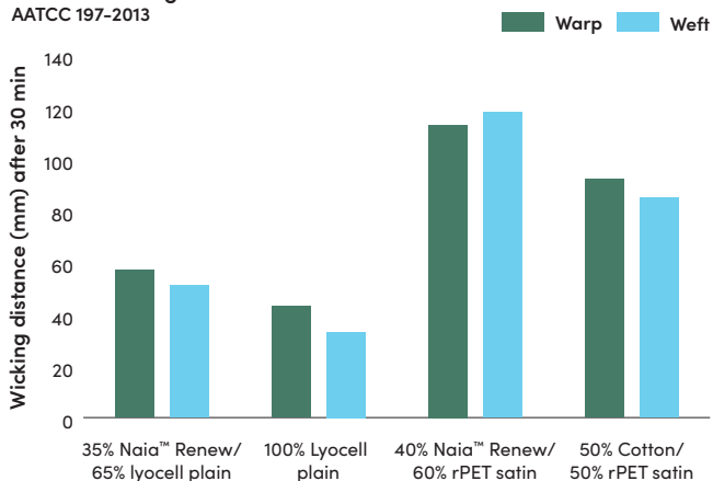
Vertical wicking AATCC 197-2013
